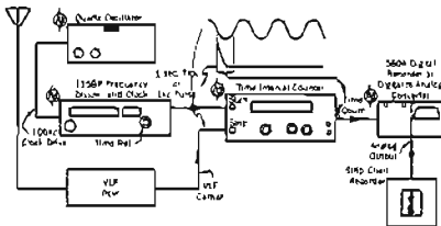
Figure 2. VLF frequency using 115BR Frequency Divider, Clock and digital electronic counter.
