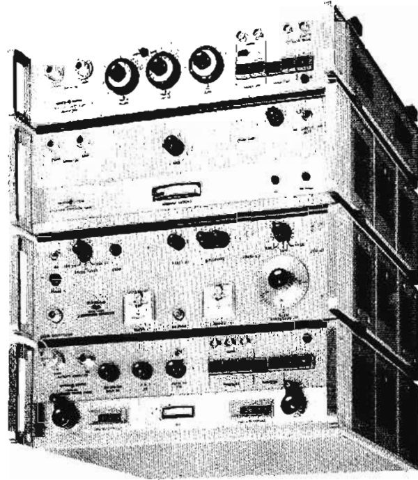
Figure 1. This hp signal generator system provides a 1 watt output with amplitude or pulse modulation. Frequency stability is 1 \times 10^{-7}/\text{sec} , 1 \times 10^{-6}/\text{week} ; P.R.F.'s to 1 mc, 20 nsec rise and fall time.
