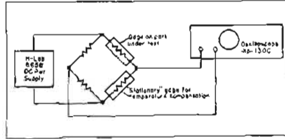
Figure 2. Dynamic strain measurements made with high-sensitivity oscilloscope.
