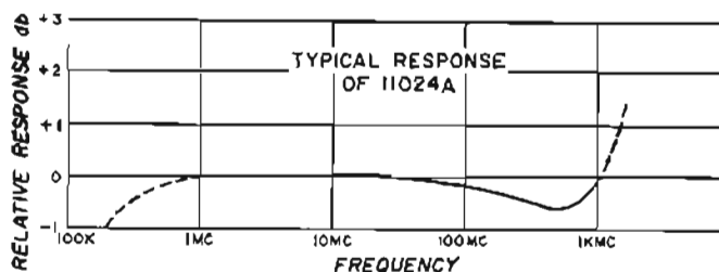
Figure 2. Typical frequency response of \text{\textcircled{4}} 11024A Type N "T" Probe Tip.
