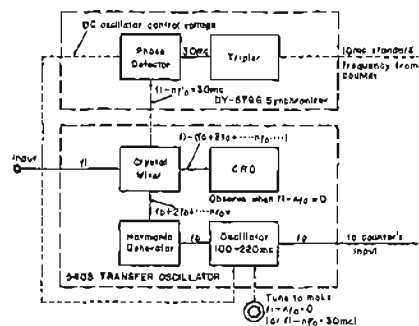
Figure 6. High frequency measurements with Transfer Oscillator. Operation is modified by addition of Dymec 5796 Synchronizer, shown connected by dotted lines.
