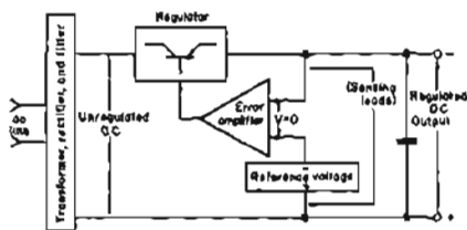
Figure 1. Regulated dc power-supply.
