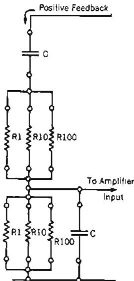
Figure 3. Frequency selective network for pushbutton oscillator.
