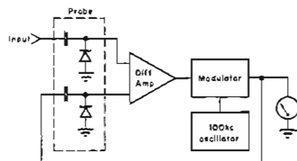
Figure 8. RF millivoltmeter.
