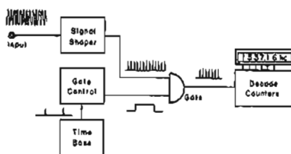
Figure 1. Frequency measurement. Function Selector is set to "Frequency" and appropriate gate time is selected by Time Base switch (combined with Function Selector on some counters).
