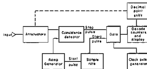
Figure 10. Simplified block diagram of 405B,C Digital Voltmeters. Decode counter overflow triggers decimal point shifter to set attenuator to higher range. No-count in hundreds counter triggers shift to lower range. On negative voltages ramp polarity is inverted.
