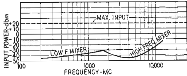
Typical Sensitivity, Model \text{Ⓢ} 540B.
