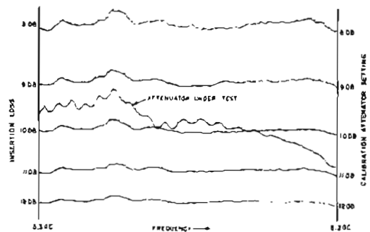
This is a typical x-y plot obtained from the setup shown in the photograph.
