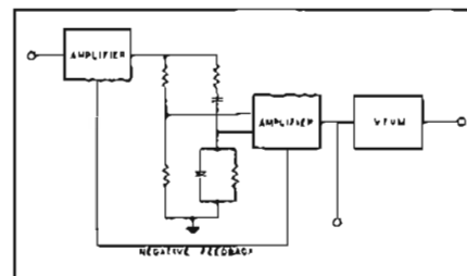
Figure 2. Block diagram of \text{HP} 330B Distortion Analyzer.
