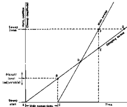
Figure 4. Representation of electron beam horizontal position vs time in oscilloscope using delaying sweep generator.
