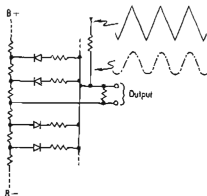
Figure 8. Non-linear shaping network.
