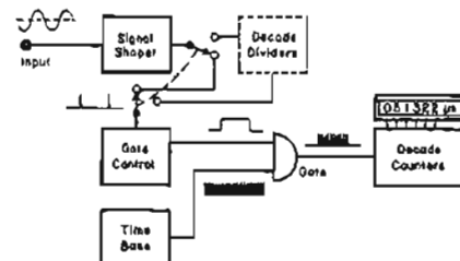
Figure 2. Period measurement. Function Selector is set to "Period" and counted frequency is chosen by Time Base switch.
