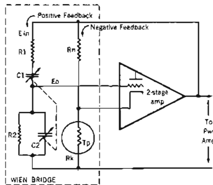
Figure 1. Basic hp Wien-bridge RC oscillator circuit.
