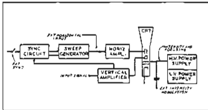
Figure 1. Simplified block diagram of an oscilloscope.
