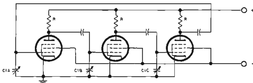
Figure 6. Phase-shift oscillator.
