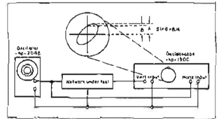
Figure 3. Phase measurement using scope in x-y mode.
