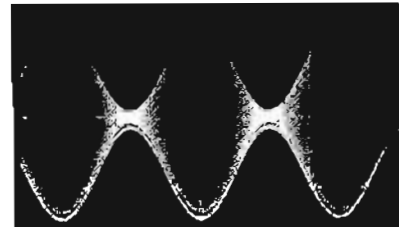
Figure 1. Dual-trace presentation comparing modulated output from \text{606A} with internal 1 KC modulating waveform (positioned closely above rf envelope).
