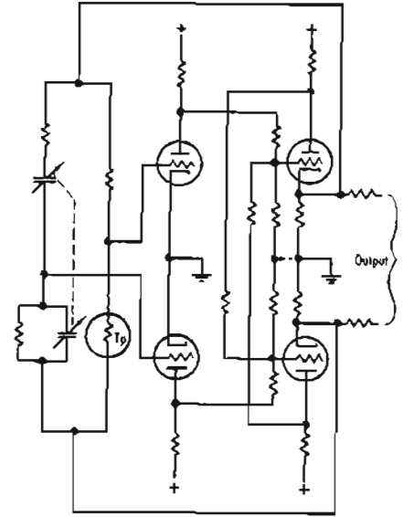
Figure 5. Push-pull RC oscillator.
