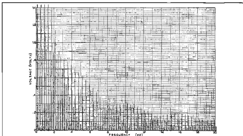
Figure 1. Harmonic analysis of slightly unsymmetrical square wave. Several harmonics were allowed to run off scale so the smaller, higher order harmonics are clearly visible.
